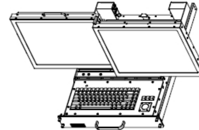
OPEN/DEPLOYED POSITION
